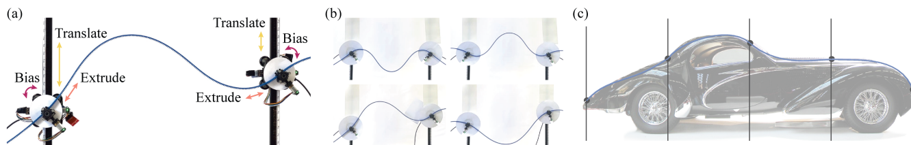
(a) Our curved line display and its degrees of freedom. (b) Four examples of curves it can create. (c) A physical simulation of a multi-segment display creating the shape of the top of a Talbot-Lago T150C.
